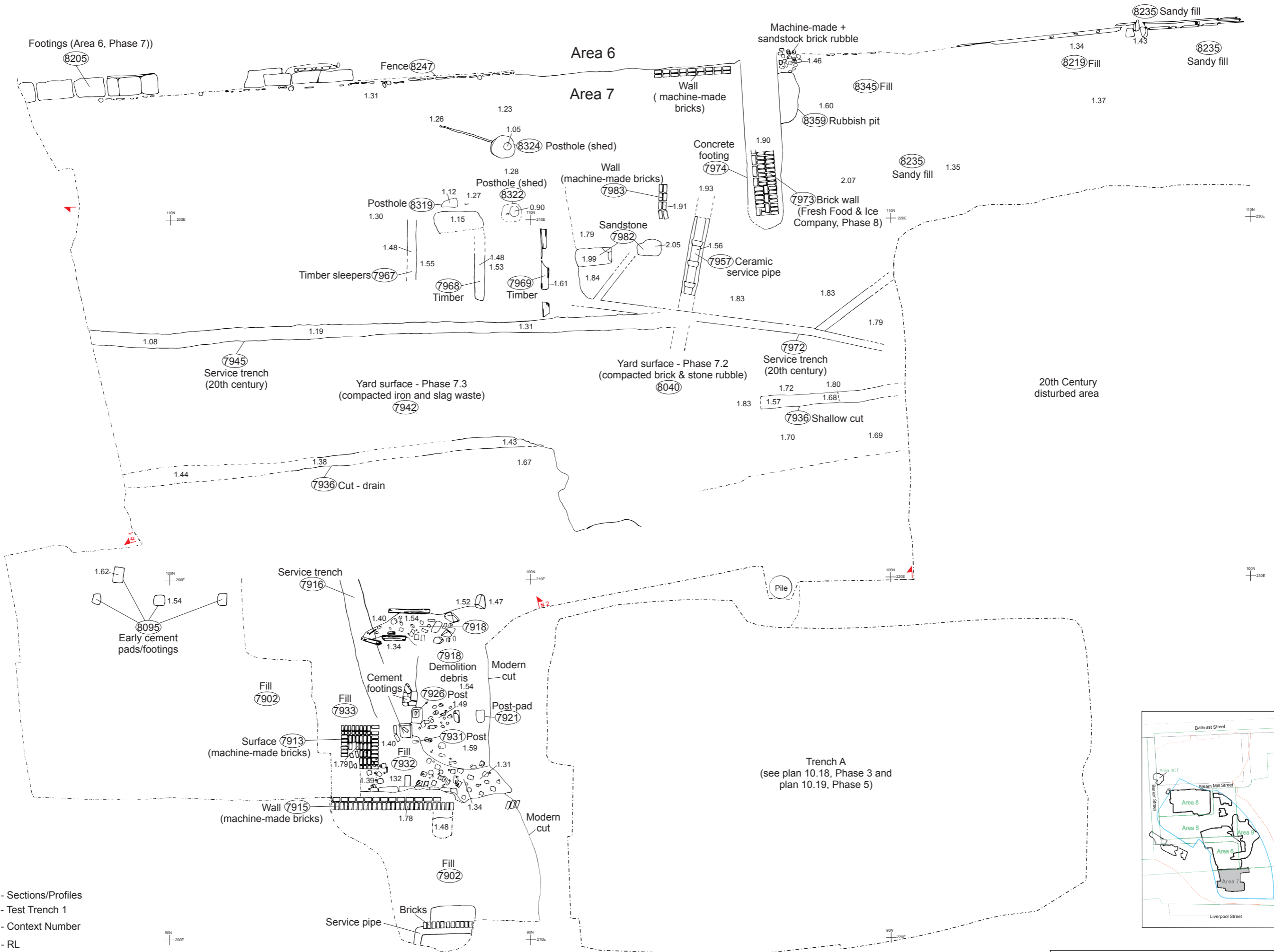
Plan 10.21: Area 7 - Phases 7.3 & 8 1880s to 1920s structures, levelling and services.
